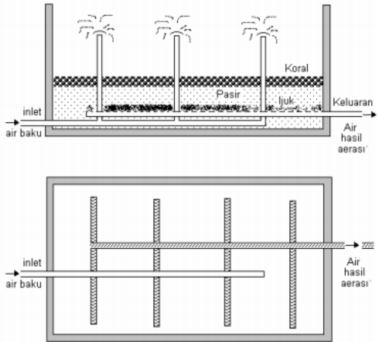
Gambar 7. 4. Spray aerator
