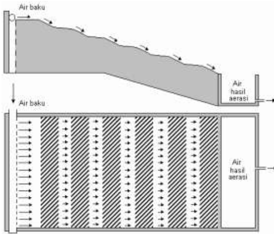
Gambar 7. 3. Submerged Cascade Aerator
