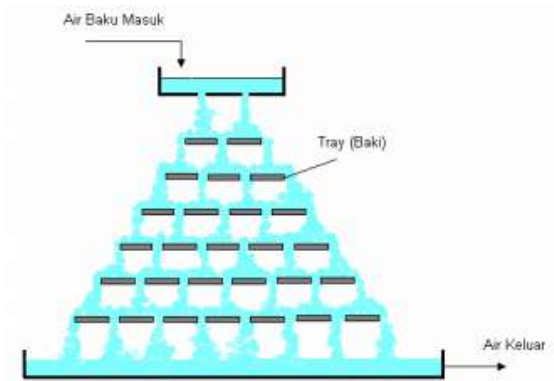
Gambar 7. 1. Tray Aerator
