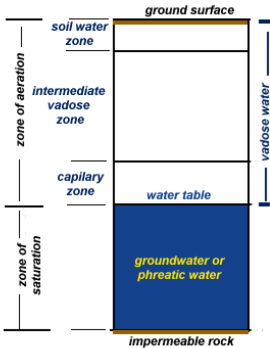
Gambar 2. 5. Distribution of subsurface water
