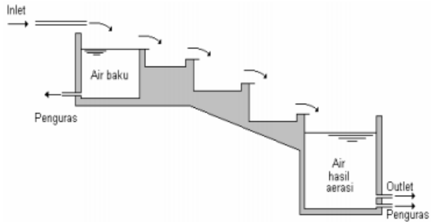
Gambar 7. 2. Cascade Aerator
