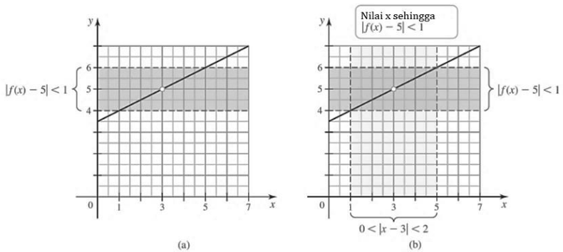
Gambar . 6.4 \lim_{x \rightarrow 3} f(x) = 5 .
