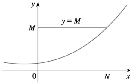
Gambar. 6.20 \lim_{x \rightarrow \infty} f(x) = \infty
