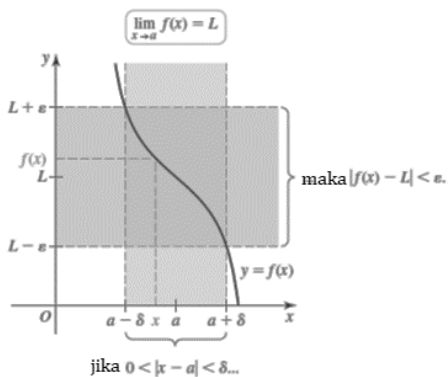
Gambar. 6.6 Jika 0 < |x - a| < \delta maka |f(x) - L| < \varepsilon
