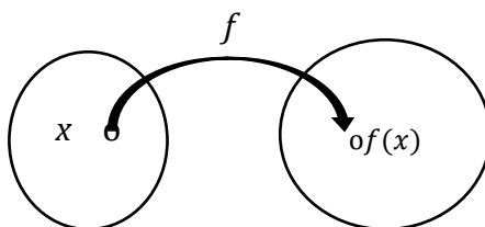
Gambar. 2.1 Diagram panah fungsi f
