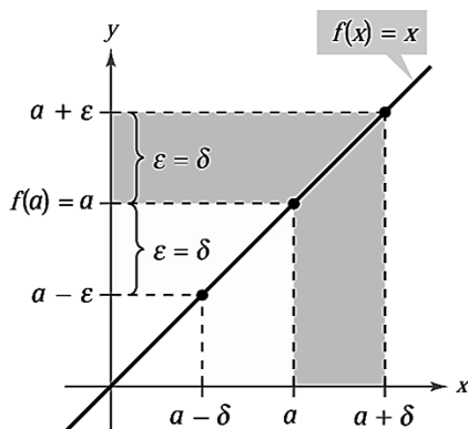
Gambar. 6.9 |x - a| < \varepsilon jika 0 < |x - a| < \delta
