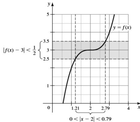
Gambar. 6.8 |f(x) - 3| < \varepsilon = \frac{1}{2}
