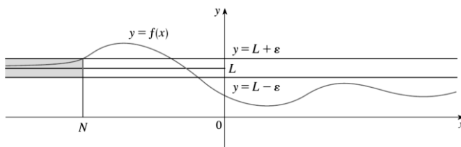
Gambar. 6.17 \lim_{x \rightarrow -\infty} f(x) = L
