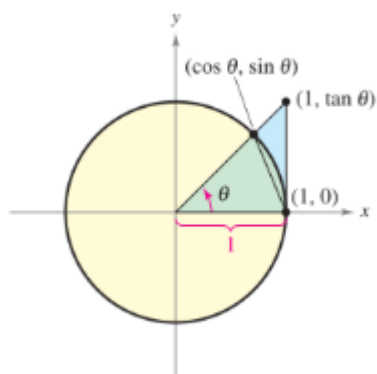
Gambar 7.6 Limit Fungsi Trigonometri
